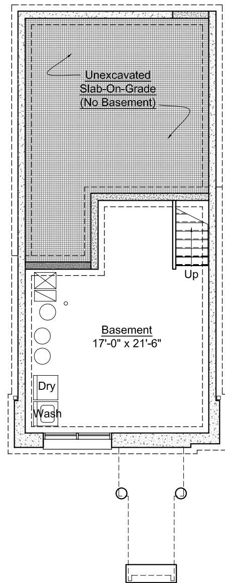
FOUNDATION/BASEMENT PLAN
