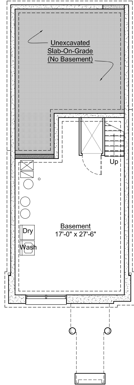
FOUNDATION/BASEMENT PLAN
